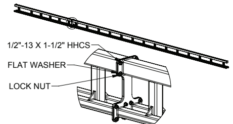
Diagram 5A. Plate style splice joint detail.
