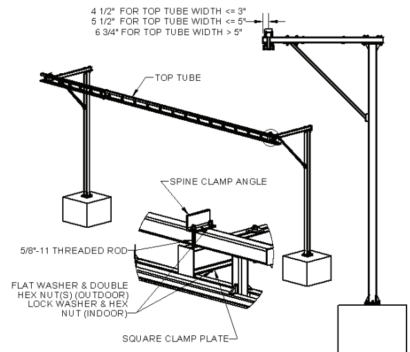
Diagram 5B. Installing threaded monorail.
