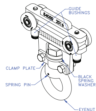
Diagram 6B. Recover trolley installation.
