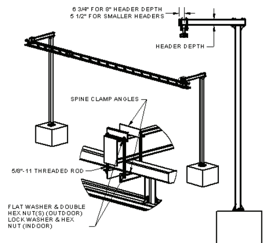
Diagram 5C. Installing under hung monorail.
