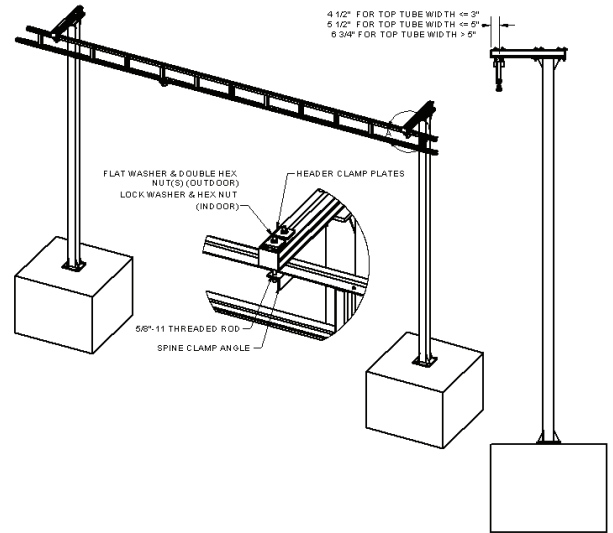
Diagram 5D. Installing Standard under hung monorail
