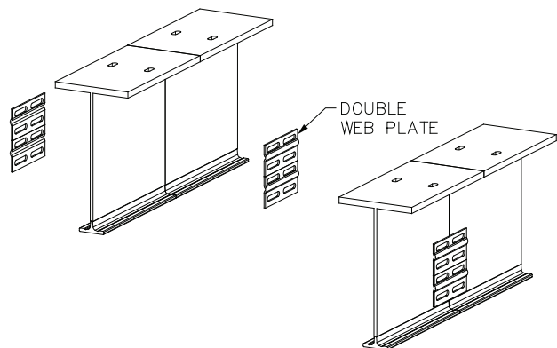
Diagram 4F. Welded splice (5000 & Larger Tarca® beam).
