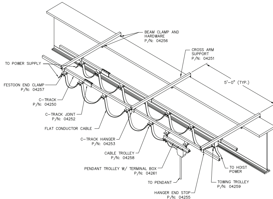
Diagram 8C. Top Flange C-Track Festooning.
