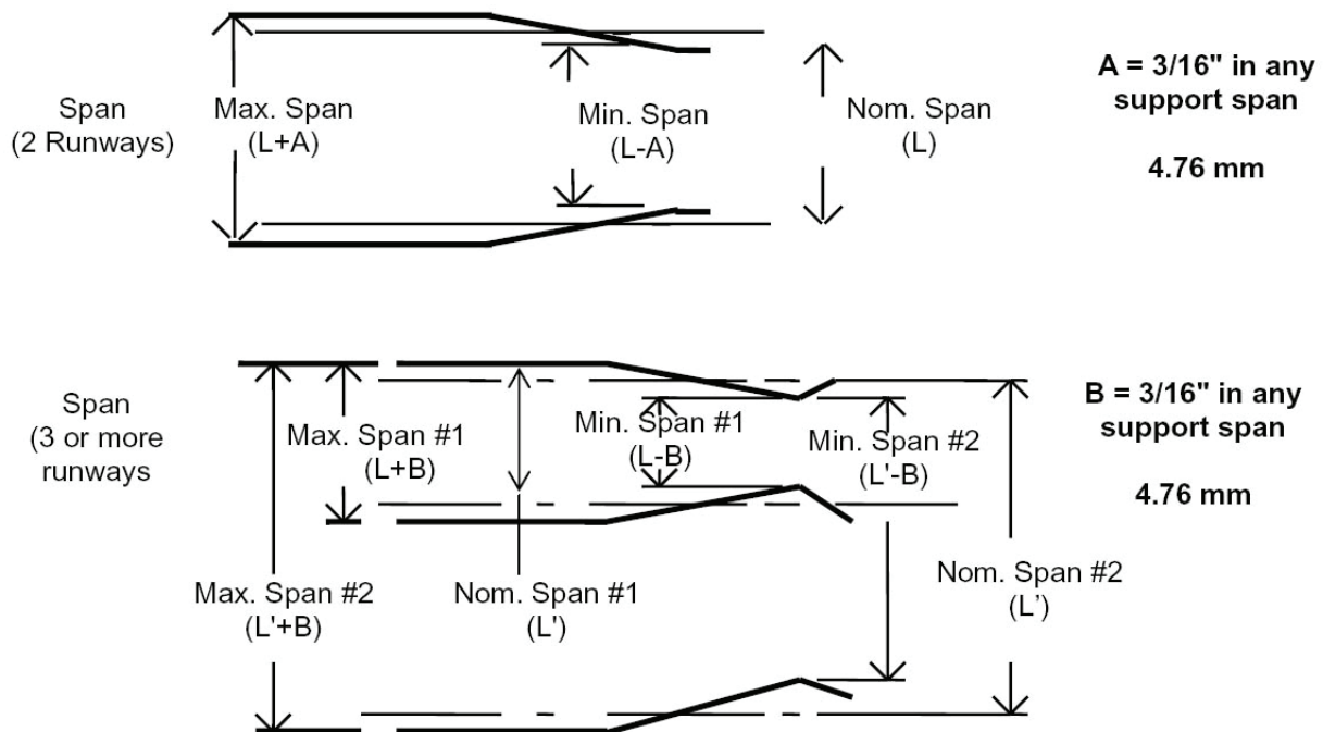
Diagram 4K. Runway alignment tolerance.
