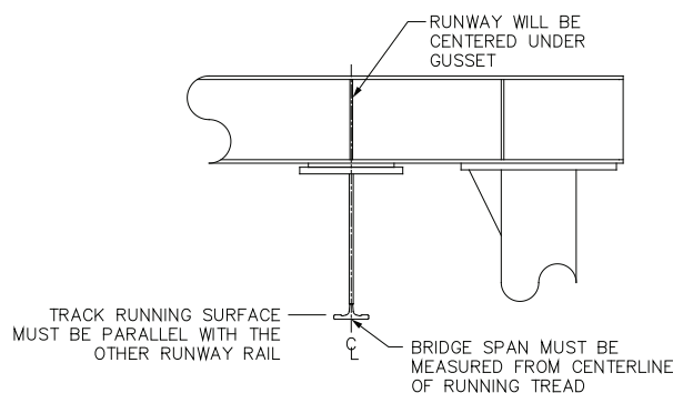
Diagram 4B. Track Perpendicularity.
